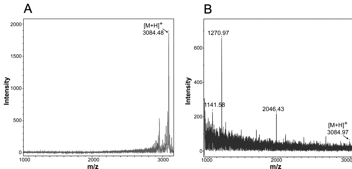
Figure 2. Mass spectrometric analysis of TED degradation products. HeLa cells were incubated with 17 \mu\text{M} TED for 15 min at 37 ^{\circ}\text{C} , and cell lysates were analyzed by MALDI-TOF MS. (A) The molecular ion at m/z 3084.48 corresponds to uncleaved TED [\text{M} + \text{H}]^{+} . (B) The molecular ion at m/z 1270.97 corresponds to cleavage of TED at the carboxyl end of the Tyr at position 8. The molecular ion at m/z 1141.58 corresponds to TED cleavage both at the Tyr residue and the N-terminal Lys residue, and the molecular ion at m/z 2046.43 corresponds to the peptide from cleavage between the two Lys at positions 13 and 14 in the TAT sequence. Uncleaved TED molecular ion [\text{M} + \text{H}]^{+} was negligible at m/z 3084.97.
